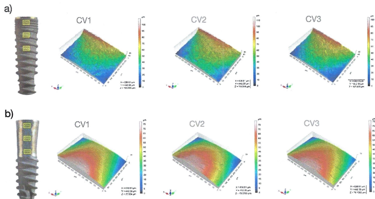
Figure 6. Confocal microscope 3D surface topography analyses of the control (a) and experimental samples (b) for each of the three regions of interest (CV1–3).
