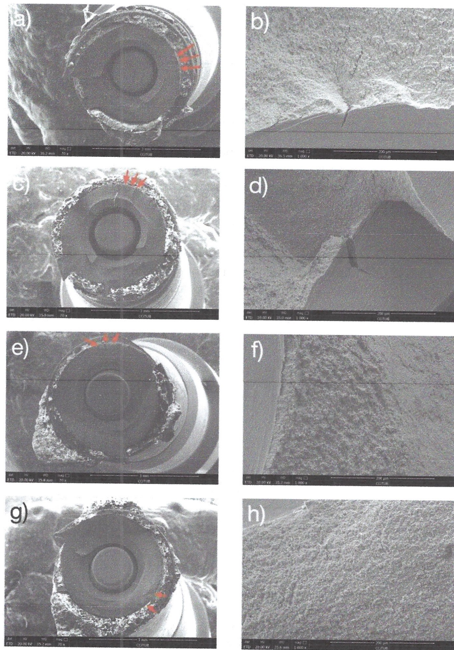
Figure 8. Fractographic analysis with scanning electron microscopy. (a–d) Control samples, a and c are macroscopic aspect of the fractured dental implants where the red arrows indicate the crack nucleation in the implant surface. b and d are the images at more magnification of a and c where can be observed the crack and the secondary cracks and their propagation. (e–h) Test samples. e and g are macroscopic images where the red arrows indicate the crack nucleation. f and h are image of the fracture surface where can be observed the ductility of the titanium.
